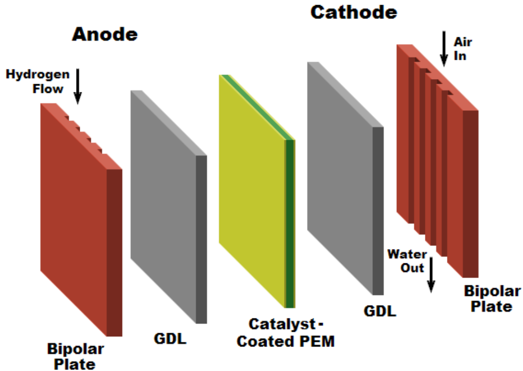
Figure 1 (above) – Exploded view of layers of PEM fuel cell. This represents one single fuel cell. For automotive applications, several hundred are stacked together.
